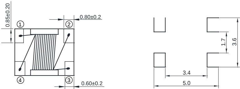
Land Pattern: [mm]
